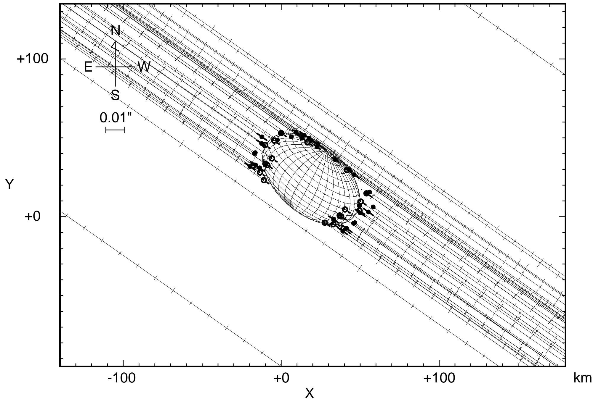
km Occultation of HIP023799 (6.2mag) by (925) Alphonsina on 2003/12/22
