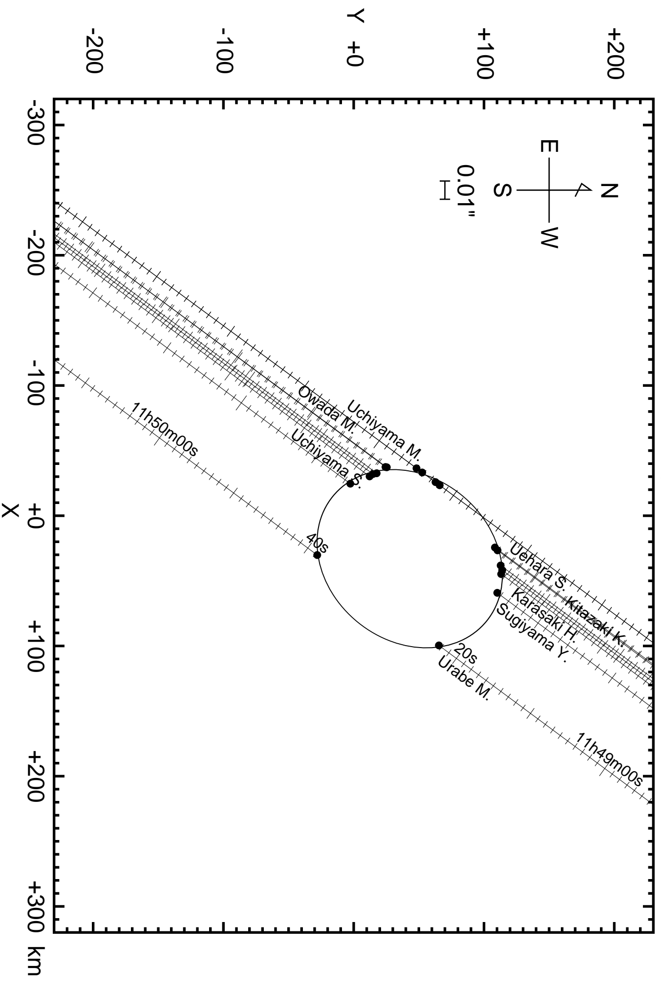
km Occultation of HIP051222 (7.1mag) by (705) Erminia on 2012/ 1/ 2
