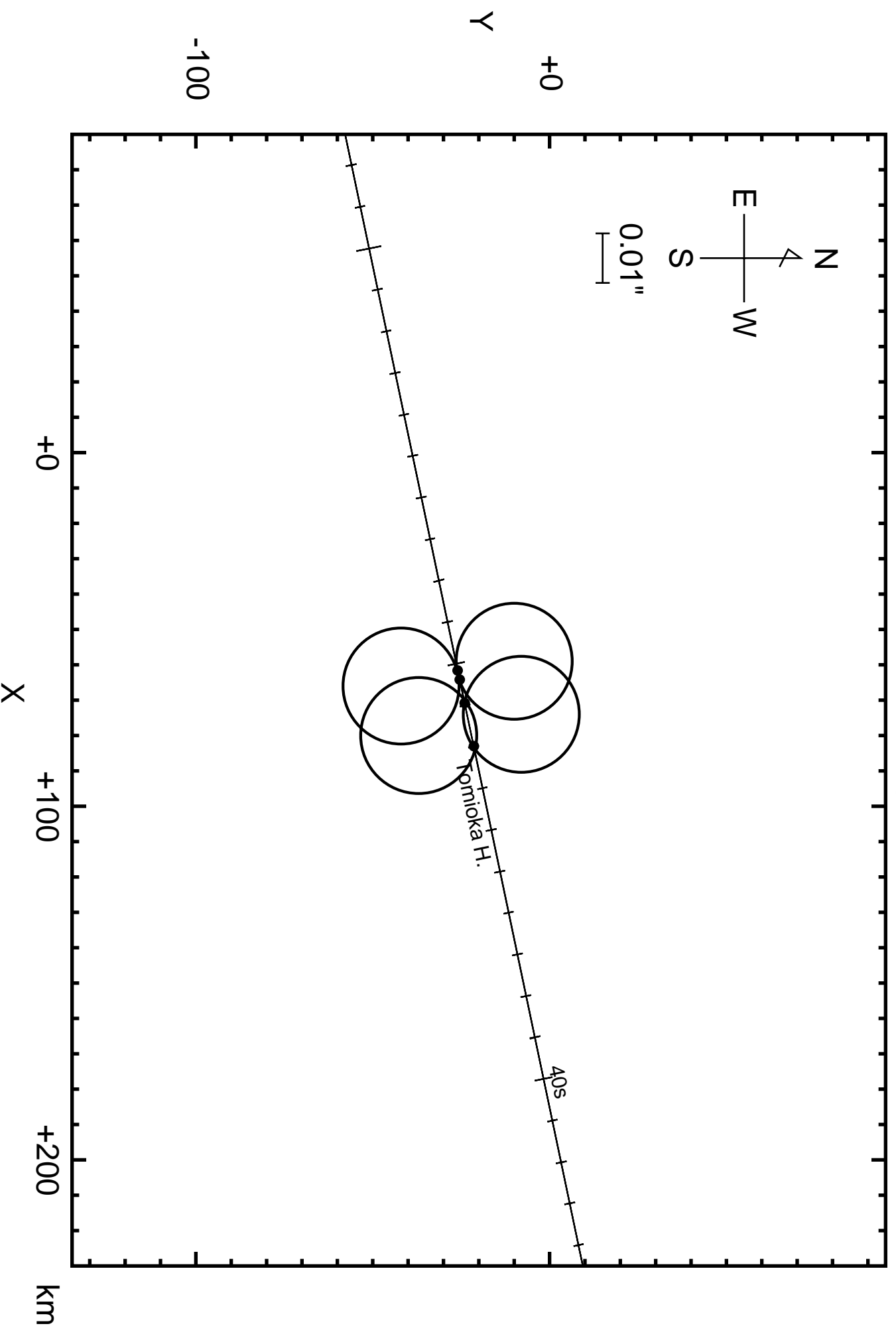
km Occultation of UCAC4_123797032 (13.1mag) by (1702) Kalahari on 2012/12/24
