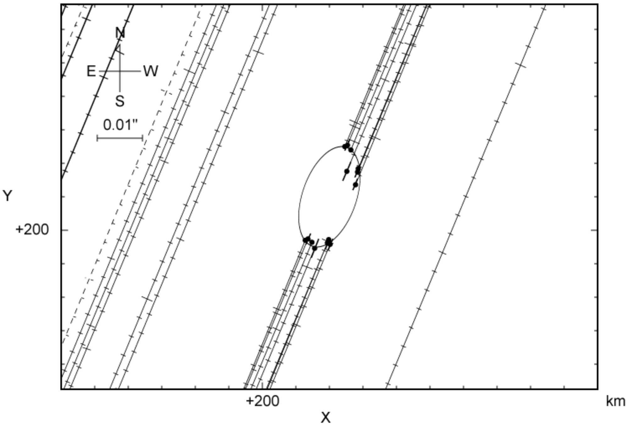
km Occultation of TYC188601206 (9.1mag) by (22) Kalliope on 2006/11/ 7
