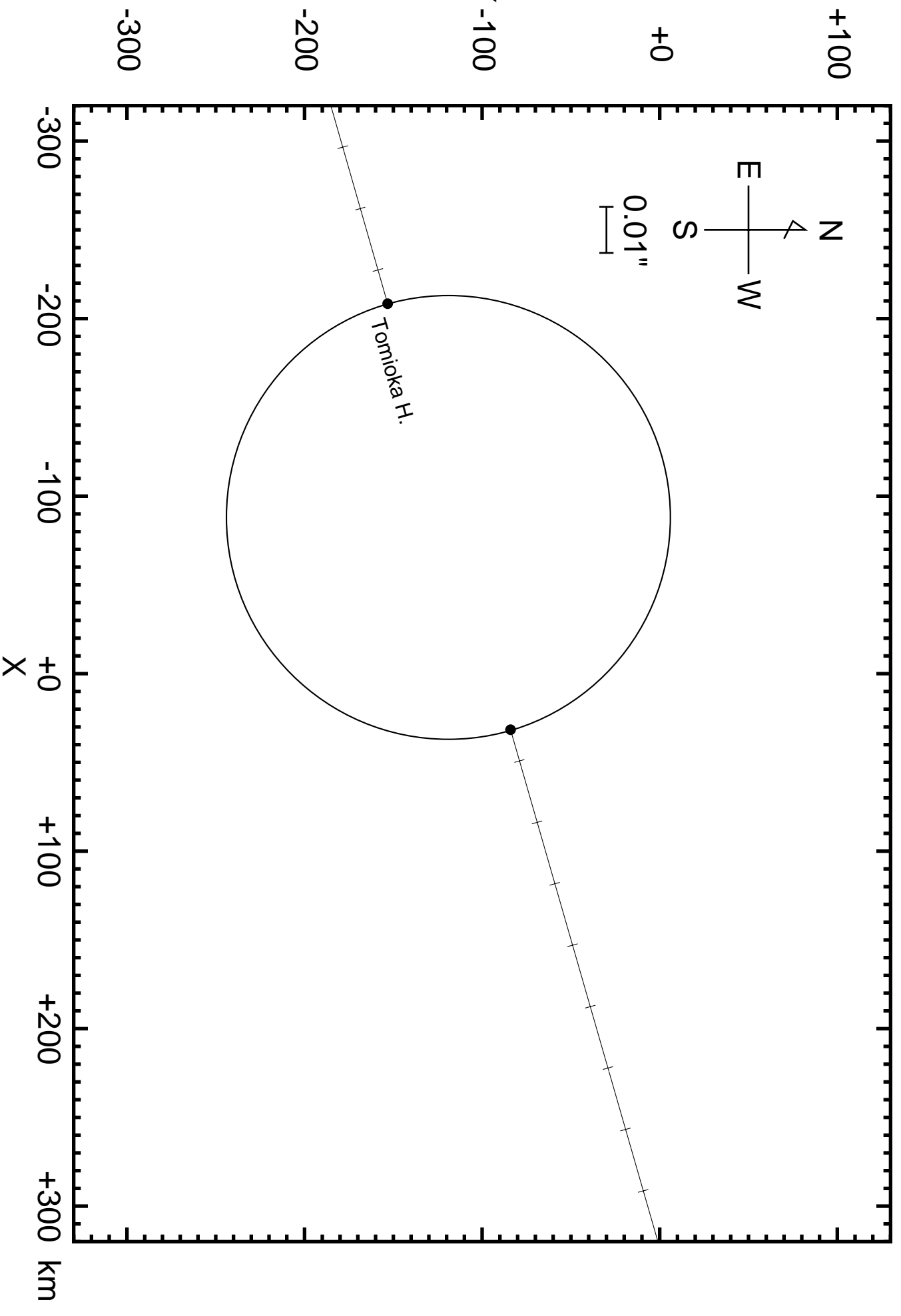
km Occultation of UCAC4_113691079 (12.1mag) by (451) Patientia on 2013/11/16
