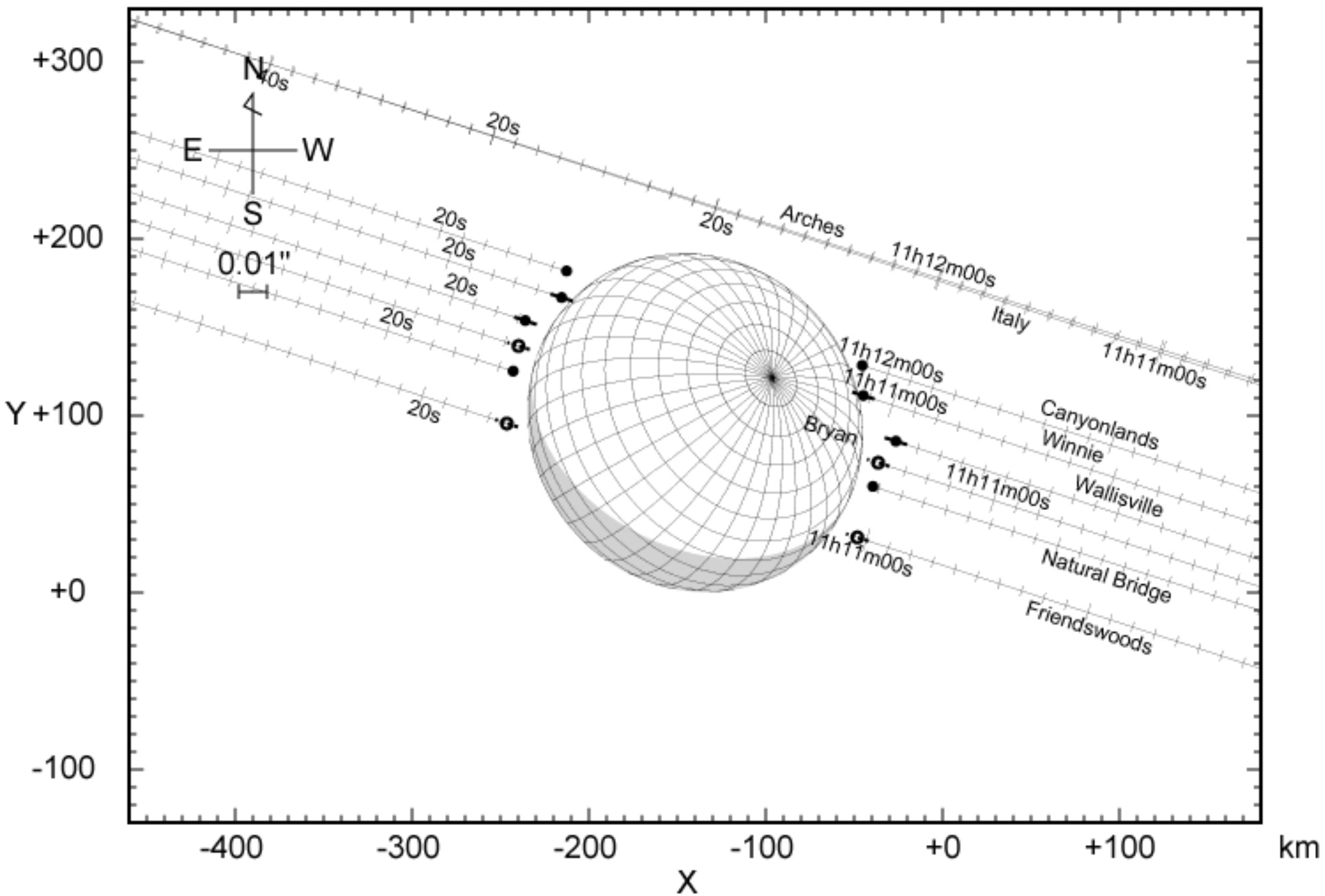
km Occultation of HIP012601 (8.8mag) by (375) Ursula on 1982/11/15
