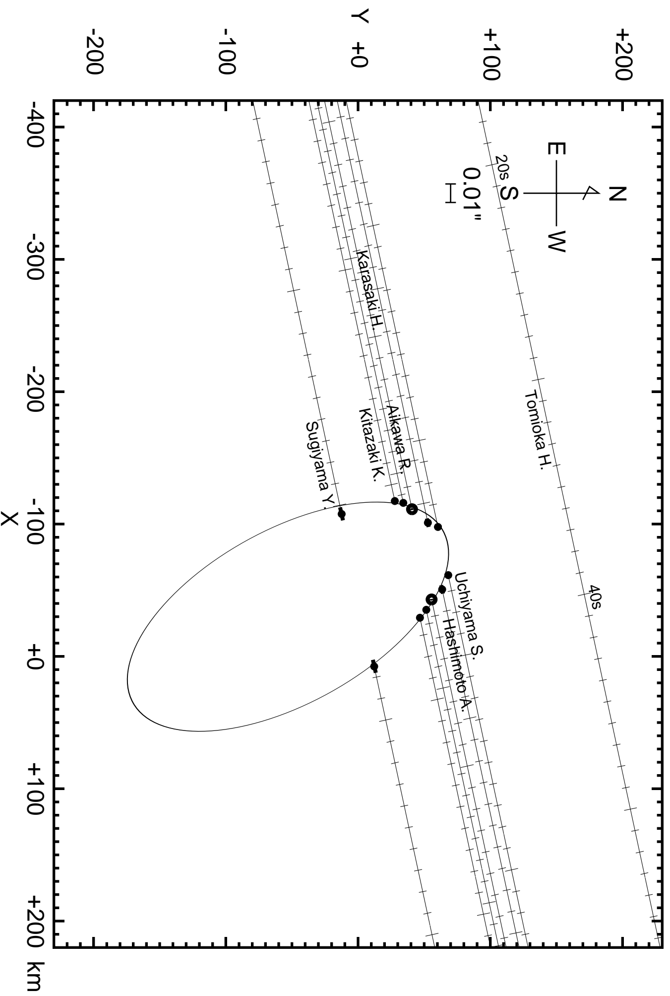
km Occultation of TYC173902256 (10.1 mag) by (654) Zelinda on 2012/ 1/ 6
